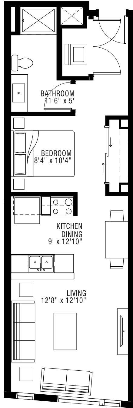
1E | FLOORS TWO & THREE
