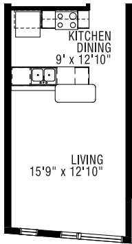
1C.4 | FLOORS TWO, THREE & SIX
